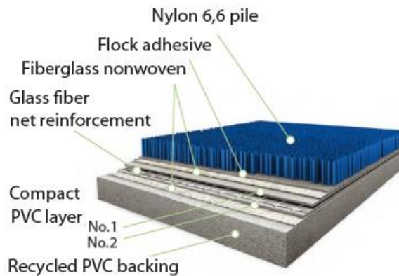
Figure 1: Typical construction
